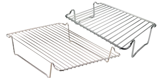
GRILL RACK* • Made from chrome plated mild steel • Suitable for all full and half size roasting tins Half size A2312 25 x 18.6 x 6.5cm Full size A2313 38 X 26 X 6.5CM
